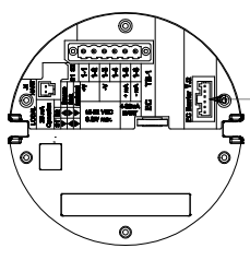
EC ADAPTER/IS BARRIER CONNECTIONS
